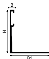
Aluminium – TRB50 B1 = 45 mm
