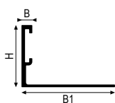
Aluminium – TRB30 B1 = 45 mm
